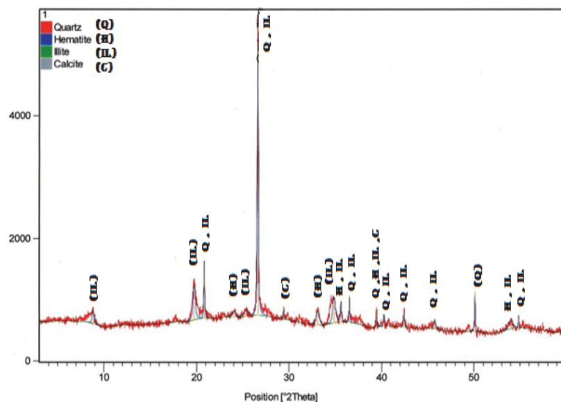
Fig. 1 Mineralogical analysis of the red clay.
