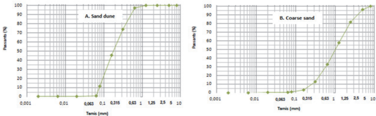
Fig. 4 Curve of particle size analysis of sand used (a-sand of dune ,B- coarse sand).
