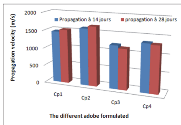
Fig. 5 Mechanical compressive strength of adobe made.
