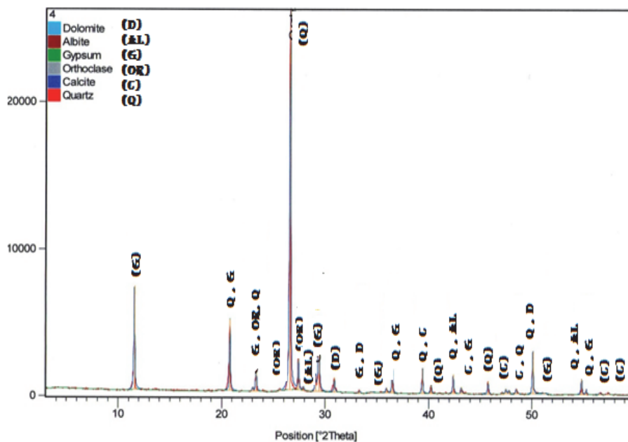
Fig. 2 Mineralogical analysis of sand dune.
