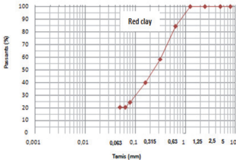
Fig. 3 Curve of particle size analysis of the red clay.
