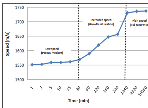
Fig. 8 Changes in the speed of wave propagation as a function of moisture.
