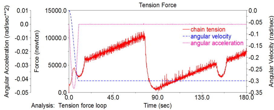
Fig. 9 Tension force loop at 0.6 friction coefficient of contact and 10 m of length with the gap is 400 mm.
