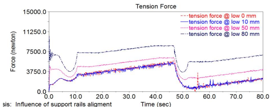
Fig. 4 Influence of supported rails alignment at 0.7 friction coefficient of contact and 7 m of length with the gap is 500 mm.
