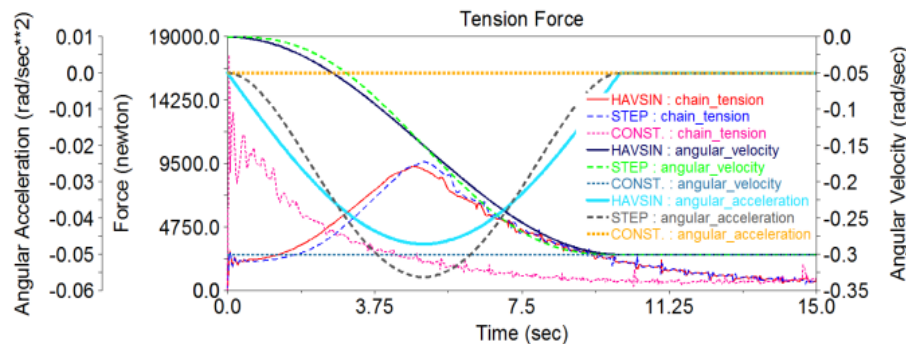
Fig. 10 Compared functions of motion between HAVSIN (time, 0, 0, 10, 0.3), STEP (time, 0, 0, 10, 0.3) and CONSTANT (0.3) as out of speed control.
