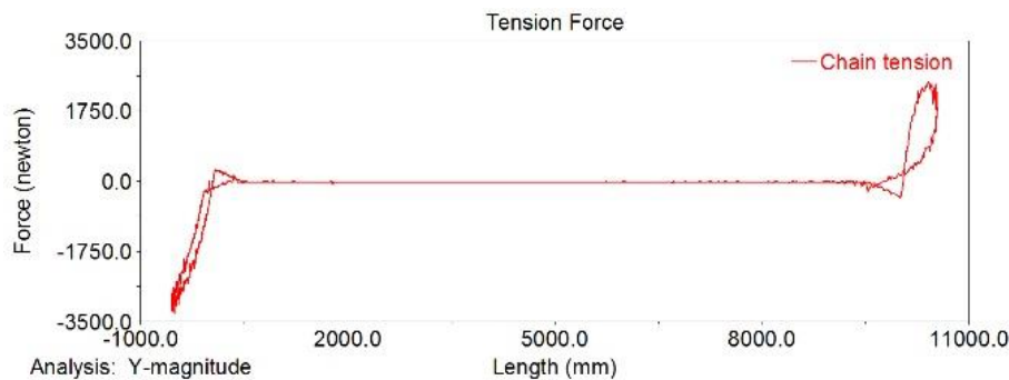
Fig. 12 Y-magnitude of tension profile vs. displacement.
