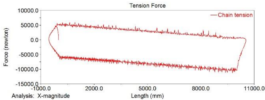
Fig. 11 X-magnitude of tension profile vs. displacement.
