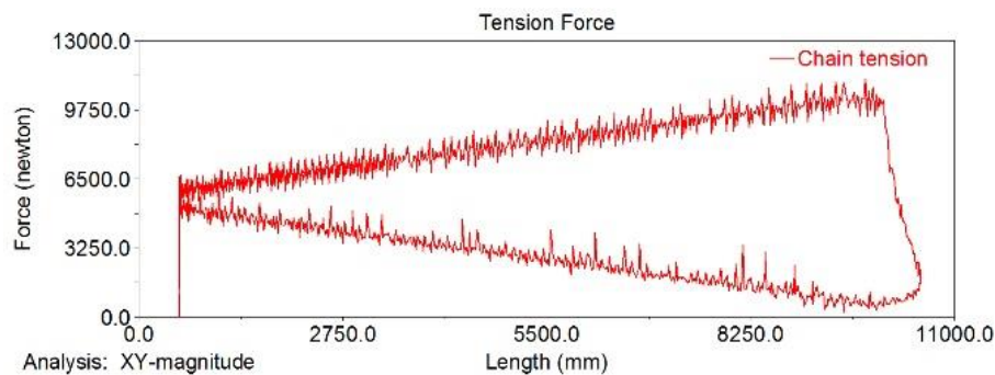
Fig. 13 XY-magnitude of tension profile vs. displacement.
